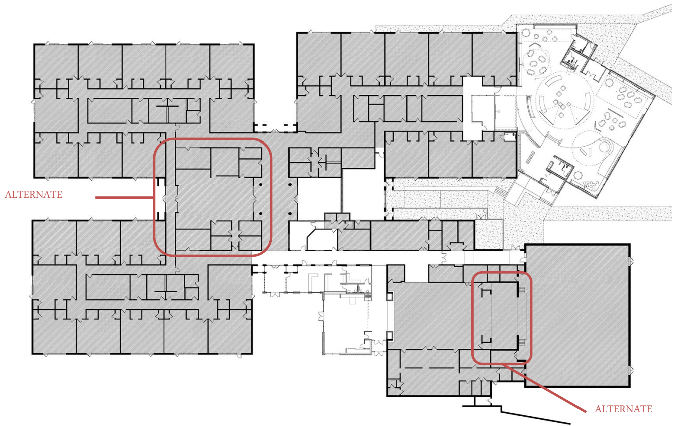
Floor Plan
